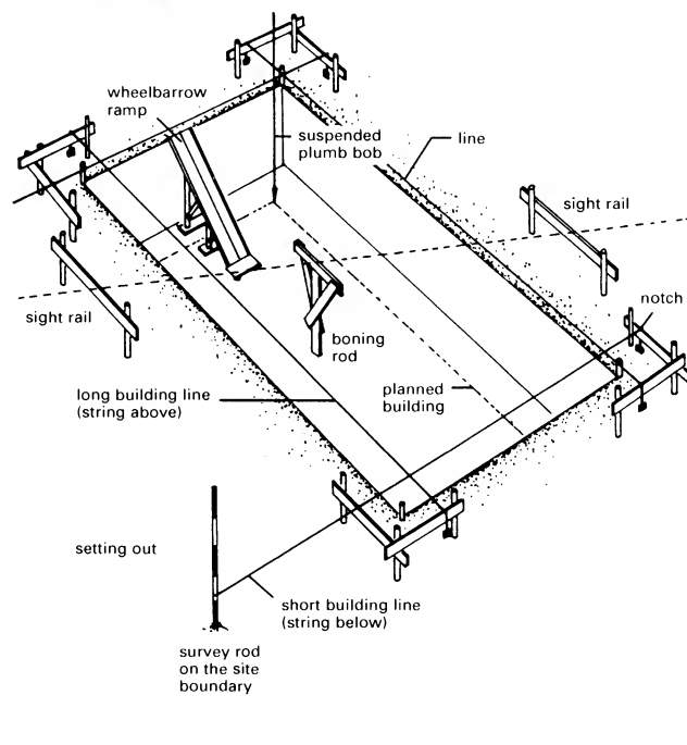
⑧ Setting out: how the building is measured into place → ⑨
